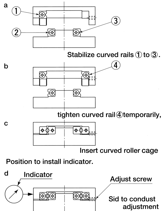
Fig. 6. Installation method (1)
