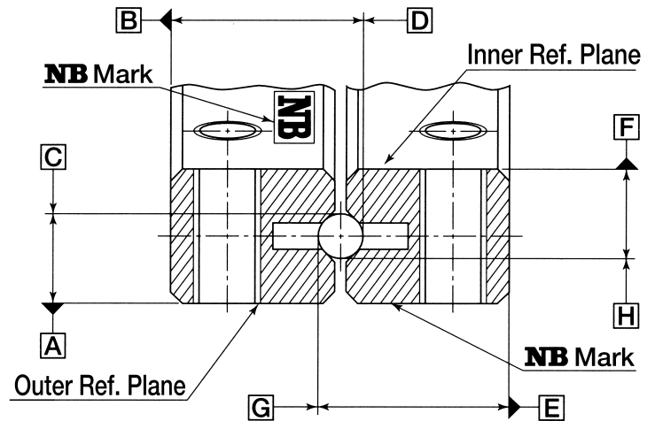
Fig. 2. Reference planes
