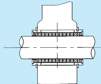
Fig.5 Use of external retaining rings
